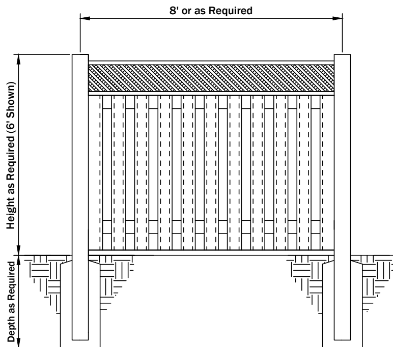
Elevation View
